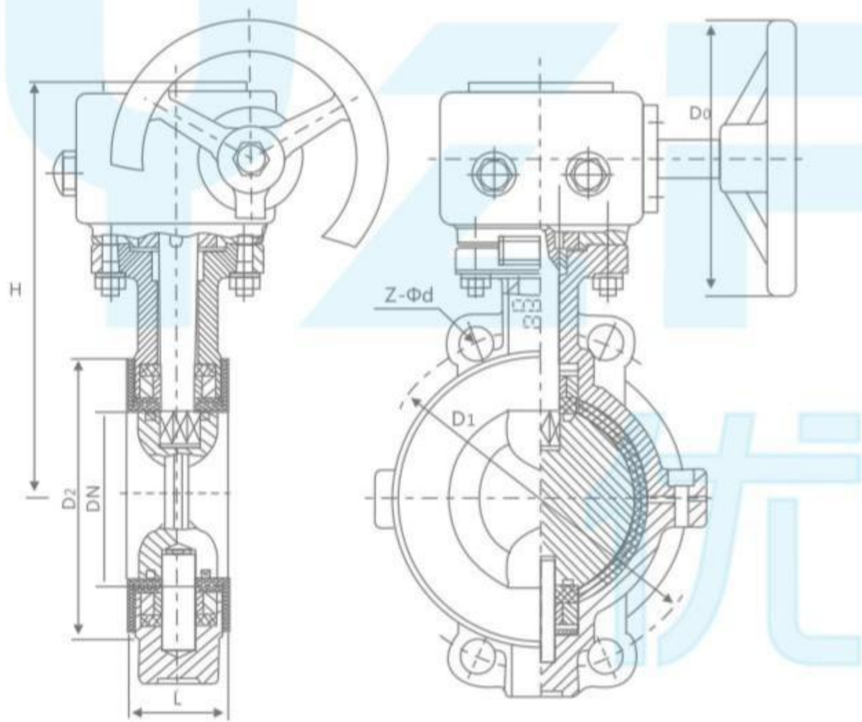
DA371 F4 F46 型对夹式蜗轮传动蝶阀 (中线) DA371 F4 F46 Wafer type butterfly valve worm gear transmission (middle)
