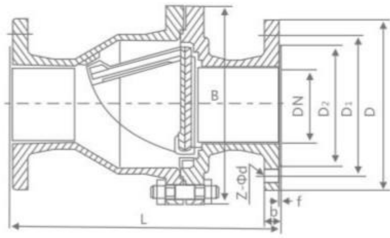
H44-F 46 F3 型止回阀(旋启式) H44-F 46 F3 Check valve (swing type)
