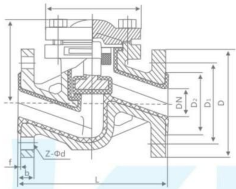
H41-F 46 F3 型法兰连接止回阀(直通升降式) H41-F 46 F3 Flange connection valve (straight-through lift)
